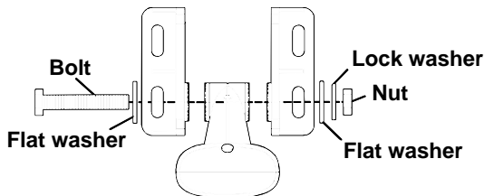
Assemble transducer and bracket.
